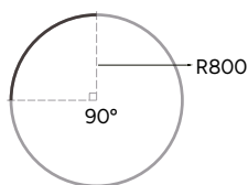
Curve Track Ø1600 mm / 90° R800
