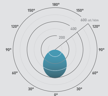
Beam angle: 100°
