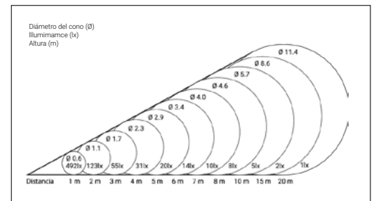
Lente W - 32° (Font Lens Focal Length = 60 mm)
