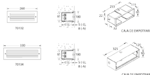
ROXY 2 MARCO INOX
