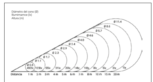
Lente W - 32° (Font Lens Focal Length = 60 mm)
