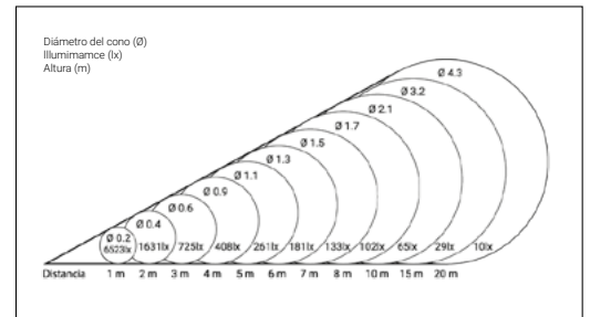
Lente M - 18° (Font Lens Focal Length = 100 mm)
