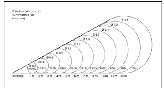
Lente M - 18° (Font Lens Focal Length = 100 mm)
